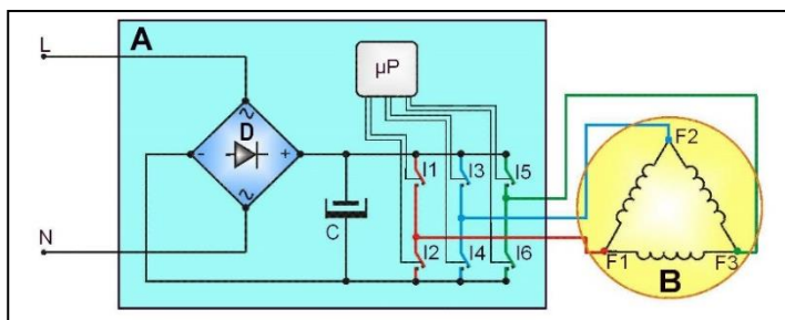
"INVERTER" operating diagram
