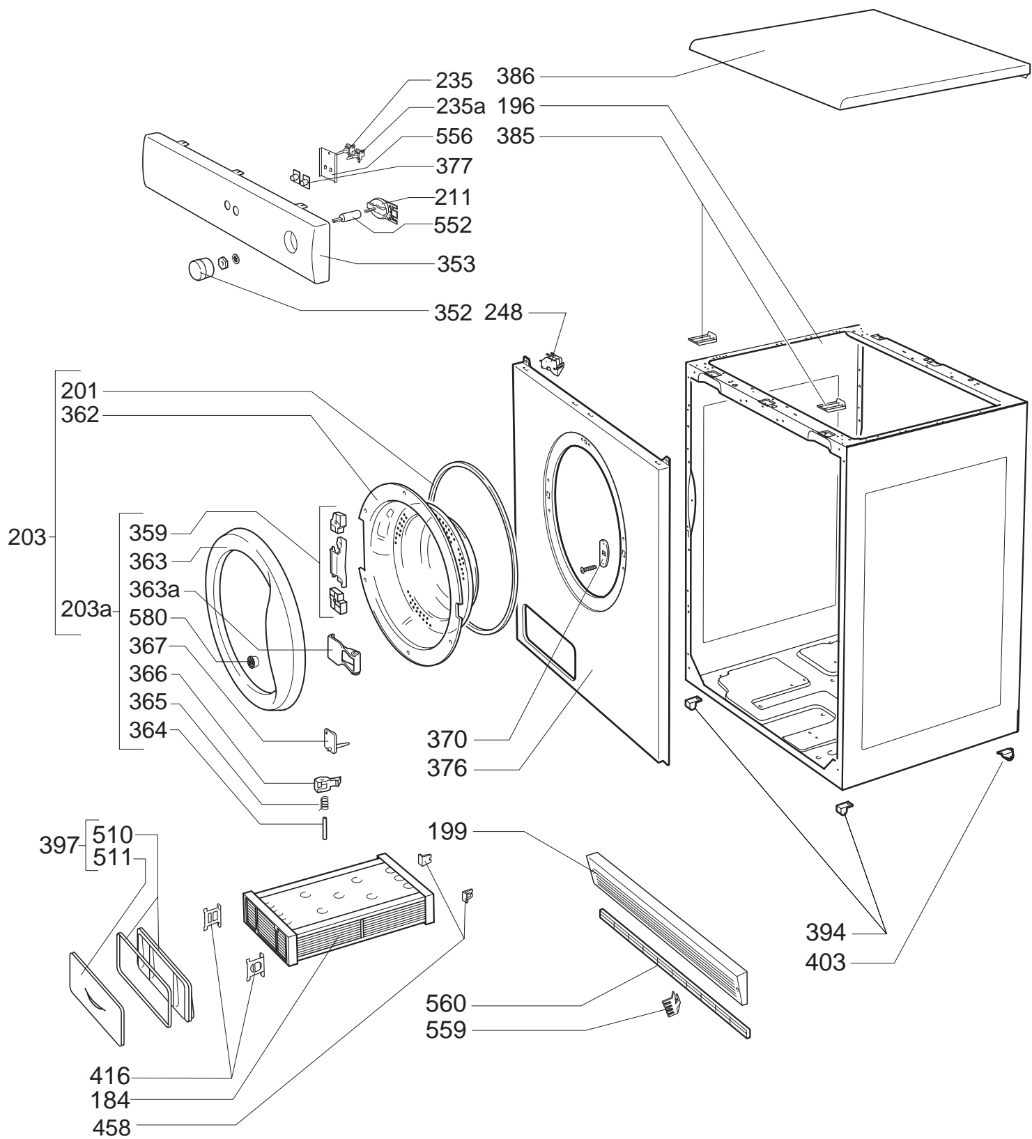
Exploded View 1
