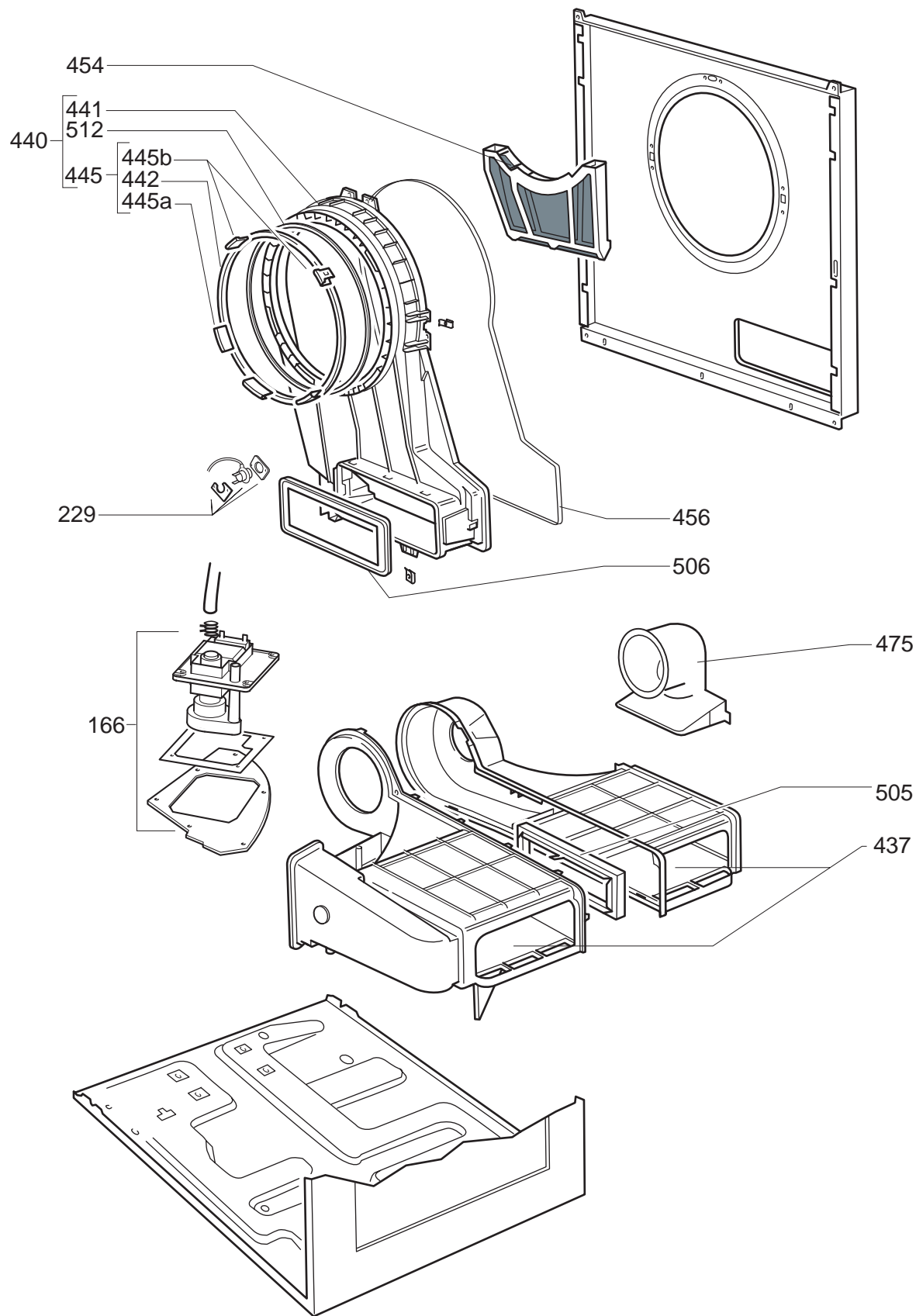
Exploded View 2
