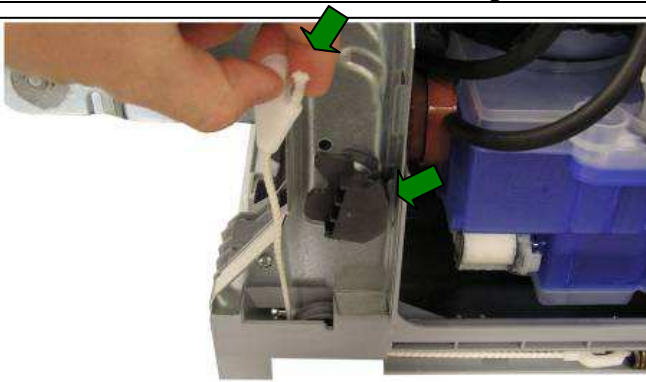
3-Now fit the clutch with the new sliding wheel..
