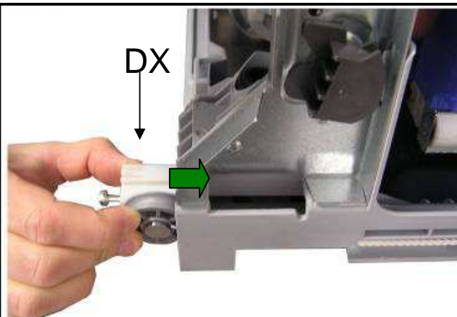
3-Now fit the clutch with the new sliding wheel..
