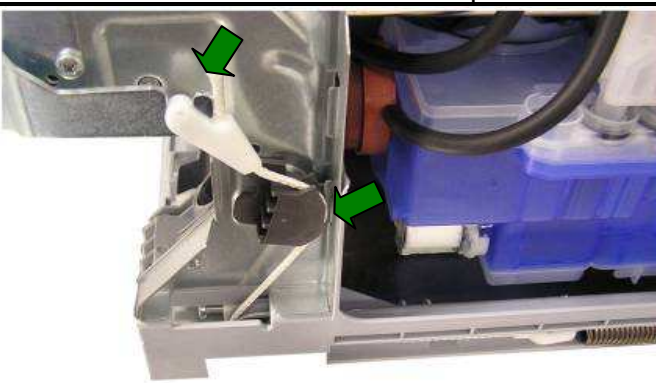
5-Adjust the screw with a Phillips screwdriver to get the proper "hardness"....
