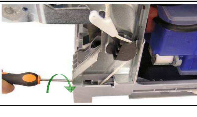
5-Adjust the screw with a Phillips screwdriver to get the proper "hardness"....
